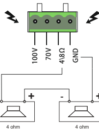
Connecting two speakers in series (8 ohm total load) to the low impedance output.
